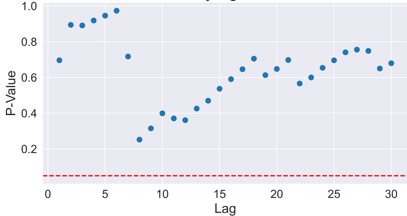
P-value from Ljung-Box test - SO2
